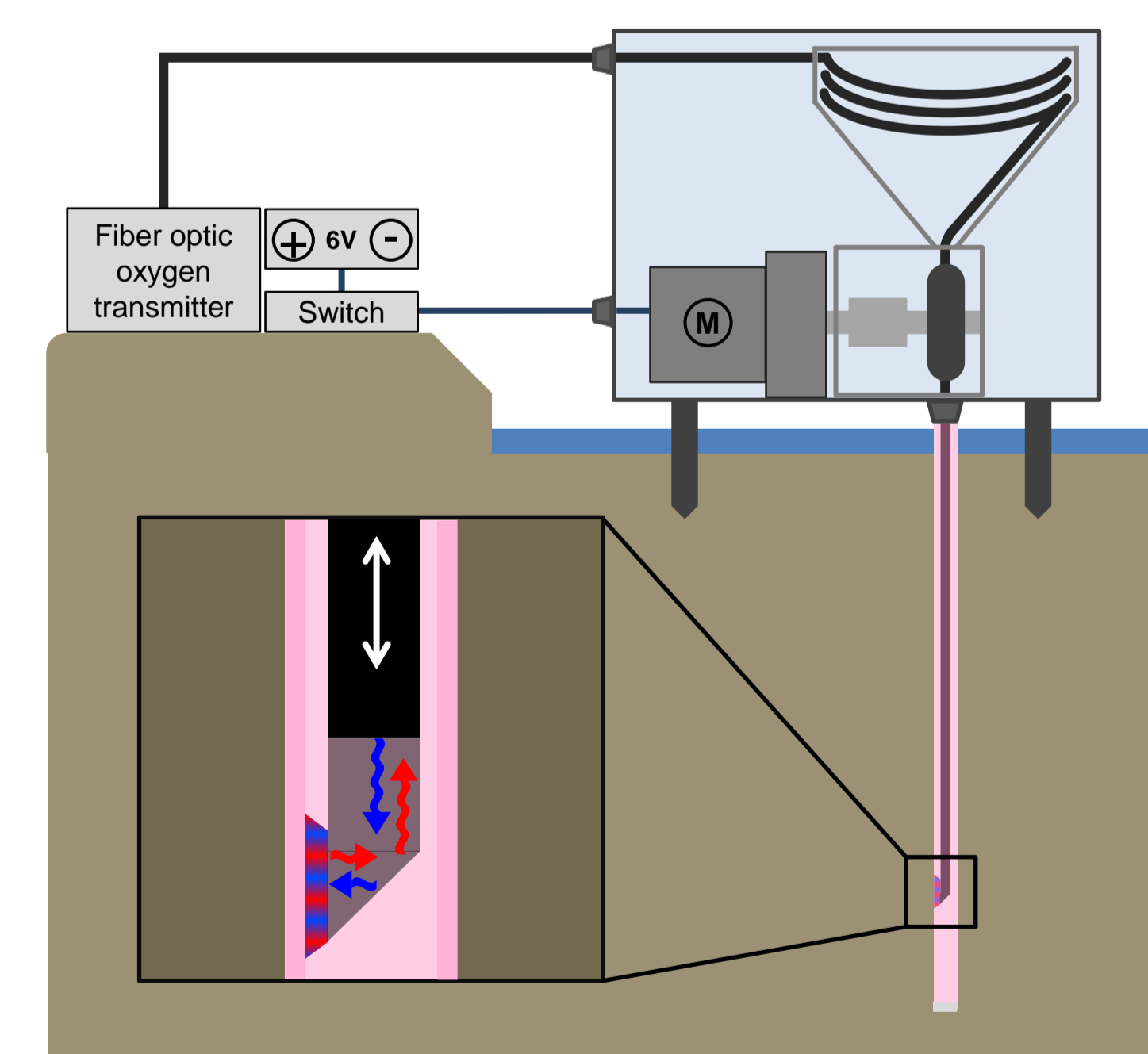
Fig. 3: Conceptual design of the miniDOS with tubular oxygen probe and control unit (not to scale).
