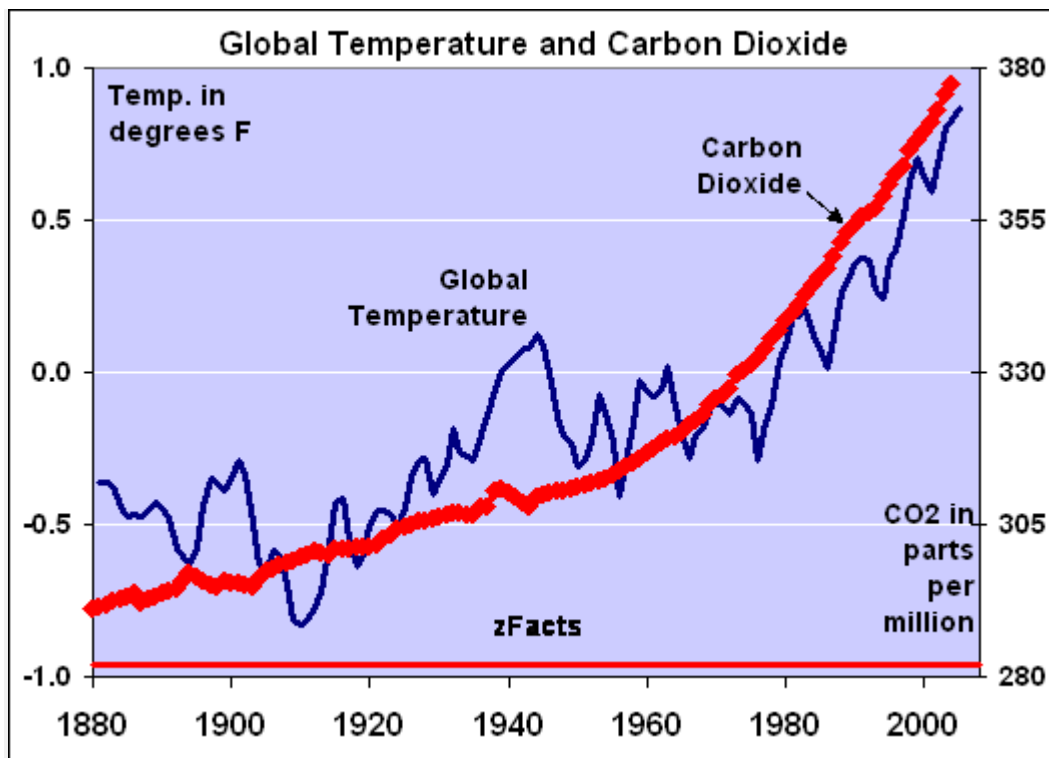
Figure 1. The average temperature of the earth and the concentration level of CO 2 in the earth's atmosphere during the 'recent' history of the last 130 years. See Stoft http://zfacts.com/p/226.html or Hocker http://wattsupwiththat.com/2010/06/09/ . A rise of 1 F is equivalent to 0.56 °C. The latter article even suggests that it is the temperature rise that is causing the increase in CO 2 concentration, not the other way round.
