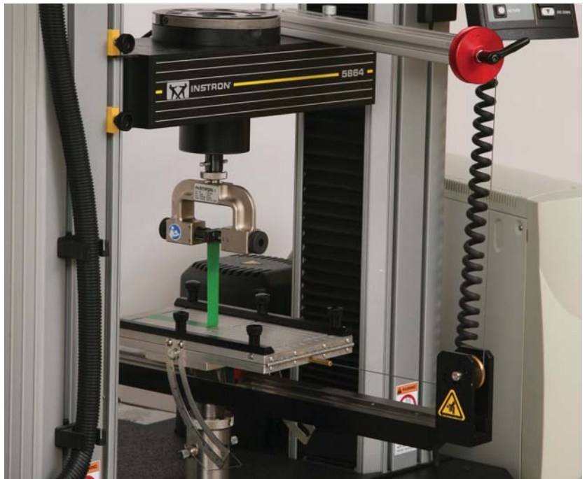
▲ 5800 Series high-speed data capture and bandwidth provide more detail in peel test results.
